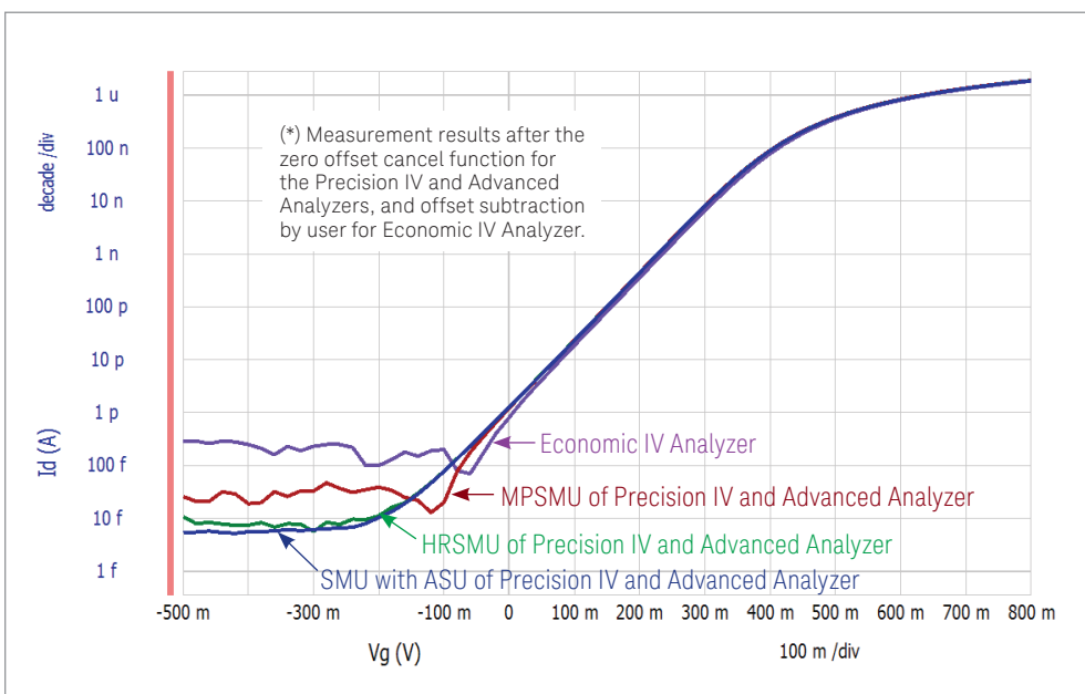
On wafer MOS FET measurement example by different SMUs
